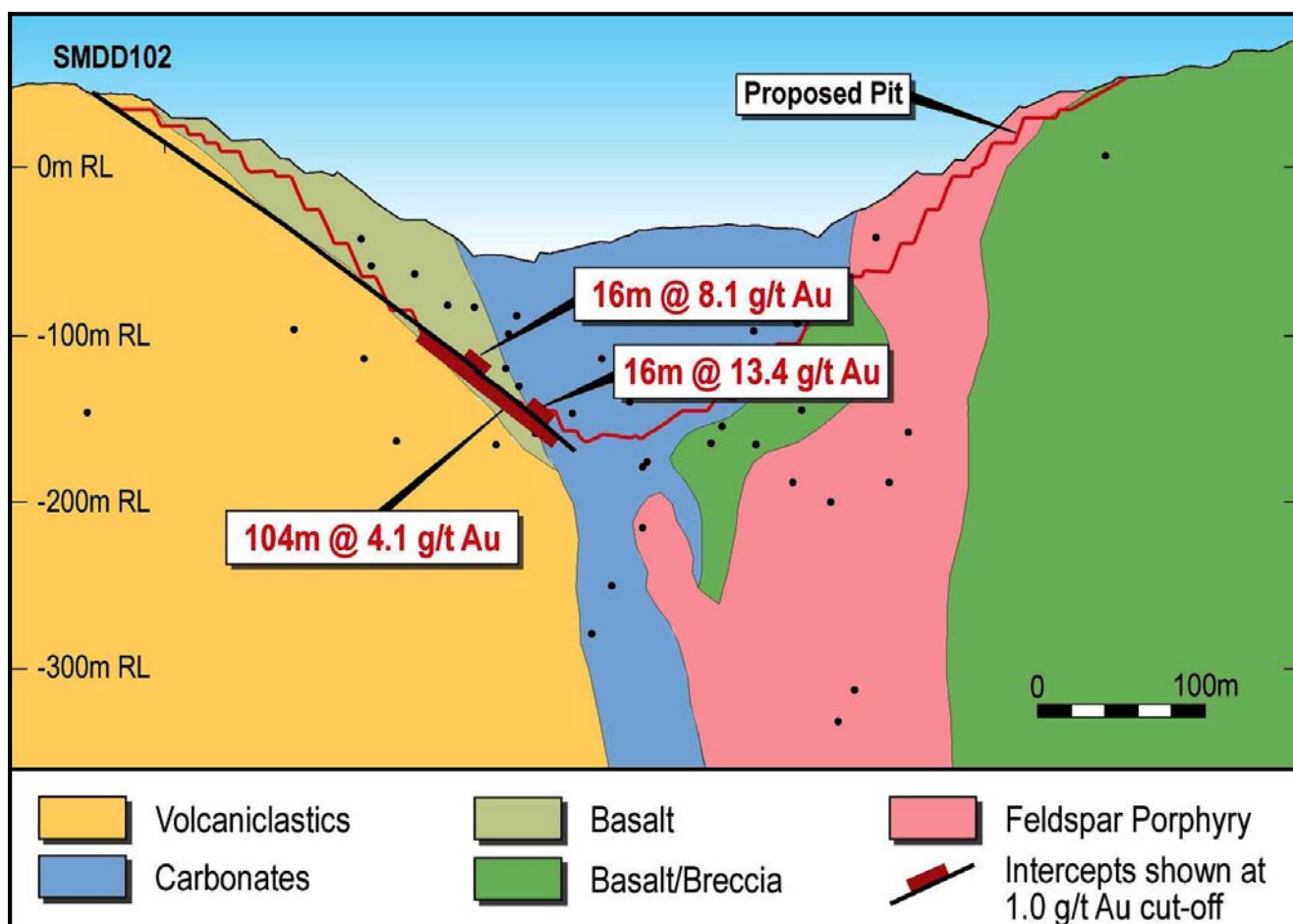
Figure 1. SMDD102 geological section in plane of drill hole (020° magnetic)
